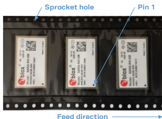
Figure 7: Orientation of SARA-R4 series modules on tape
