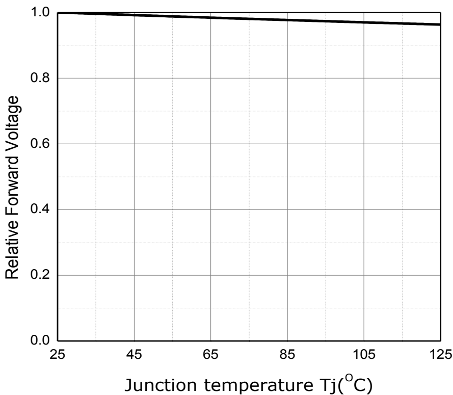
Fig 7. Junction Temperature vs. Relative Forward Voltage, I_F=65mA
