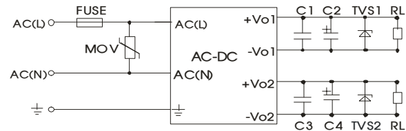
Fig. 4: LH15-10Dxx (Isolate Twin Output) series typical application circuit
