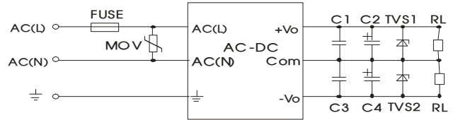
Fig. 2: LH15-10Axx (Dual Output) series typical application circuit
