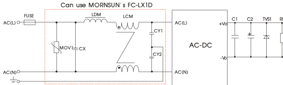
Fig 5: EMC Recommended circuit with higher requirements (Output external circuit refer to the typical application circuit)
