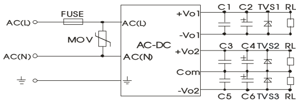
Fig. 3: LH15-10Cxx (Triple Output) series typical application circuit
