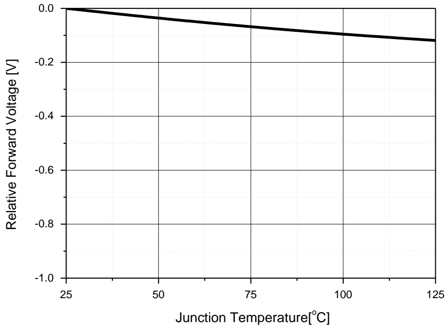
Junction Temperature vs. Relative Forward Voltage at IF=350mA
