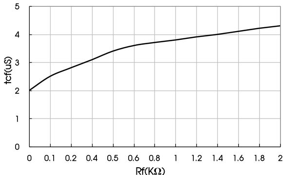
Reference curve of relation between fault soft turn-off time and R f
