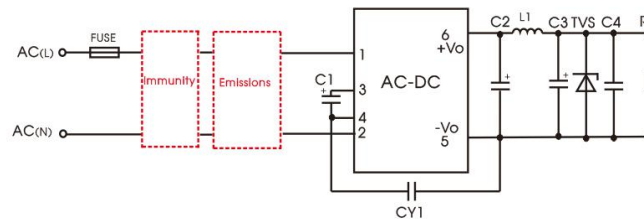
LS05 series additional components selection guide (No EMC devices)
