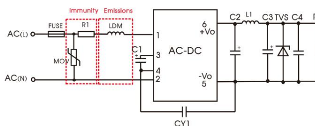
Application circuit 4
