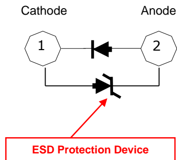
Circuit
