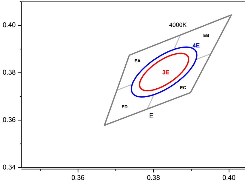
CIE Chromaticity Diagram, T_j=25^\circ\text{C} , I_f=65\text{mA}
