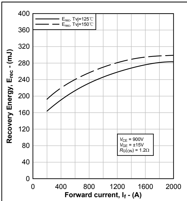
图 9. FRD 反向恢复能耗典型曲线, E_{rec} = f(I_f) Fig.9 Typical FRD E_{rec} , E_{rec} = f(I_f)
