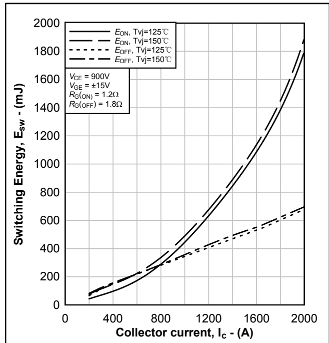
图 10. IGBT 开关能耗典型曲线, E_{on} = f(I_c) , E_{off} = f(I_c) Fig.10 Typical IGBT switching energy, E_{on} = f(I_c) , E_{off} = f(I_c)
