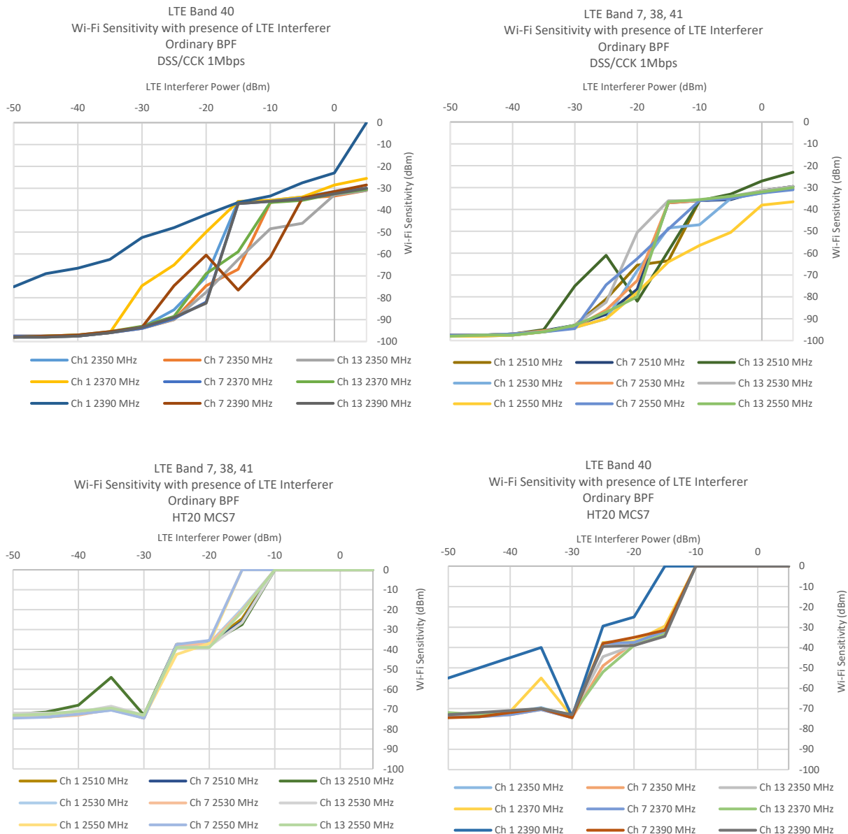
Figure 19: Wi-Fi sensitivity
