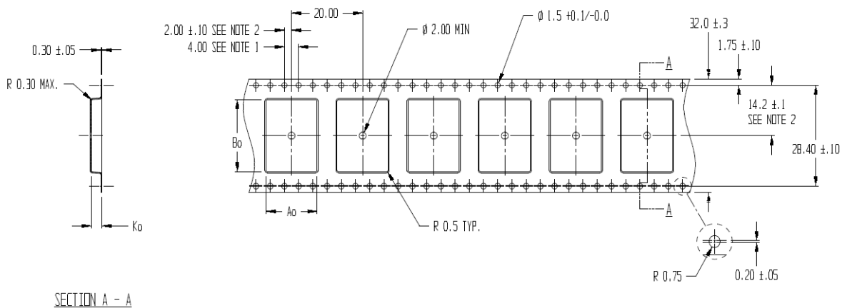
Figure 21: Orientation of JODY-W1 modules on tape
