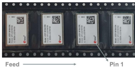
Figure 21: Orientation of JODY-W1 modules on tape
