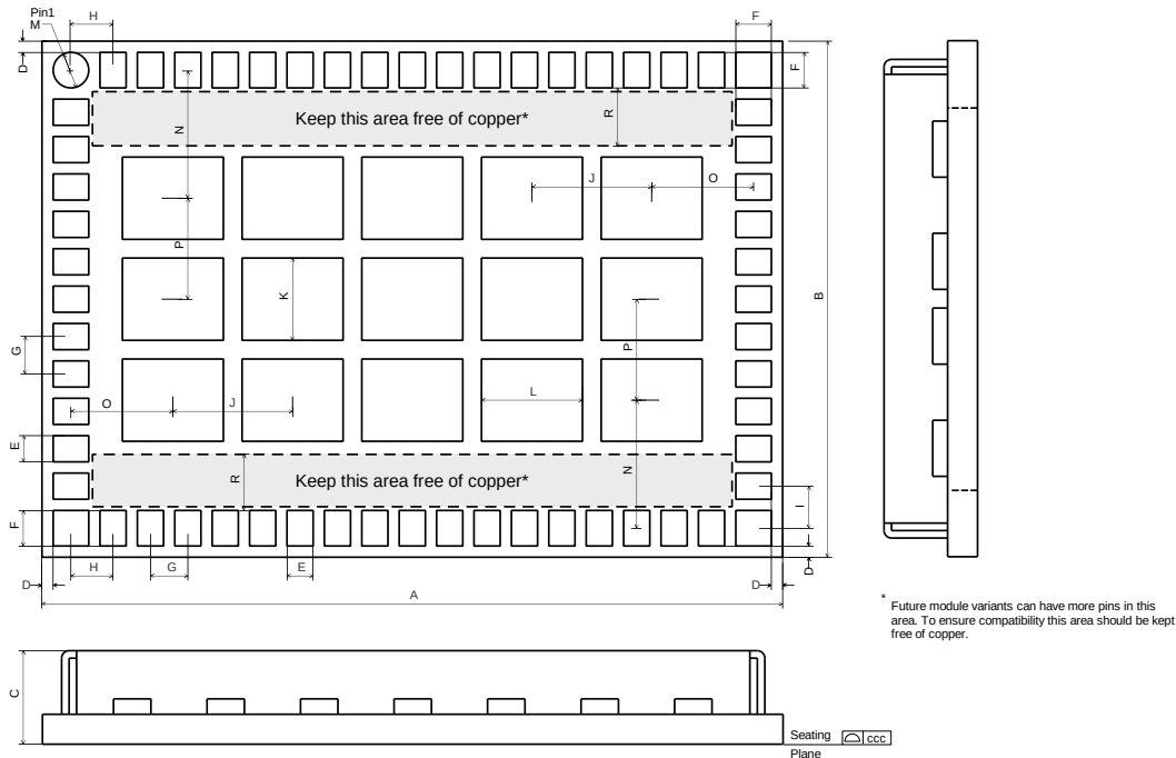
Figure 20: JODY-W1 series dimensions (bottom view)
