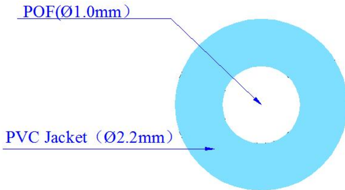
CCVt2-1000 Structure Diagram
