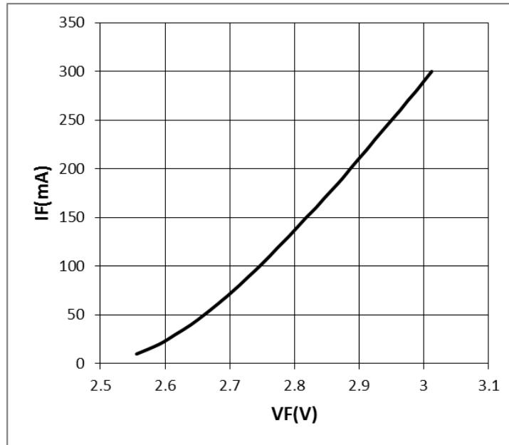
Fig 3. Forward Voltage vs. Forward Current, T_j = 25^\circ\text{C}
