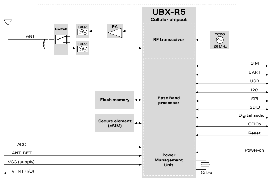
Figure 1: SARA-R500S block diagram
