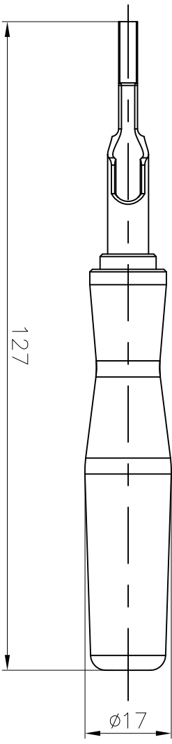
Contact removal tool Application: 16A Crimp contacts
