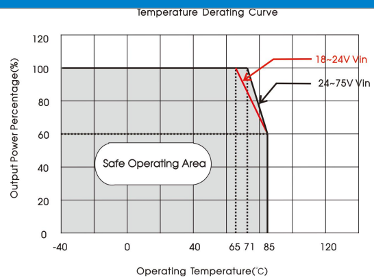
URH4803LP-20WR3, URH4805LP-20WR3 Temperature Derating Curve
