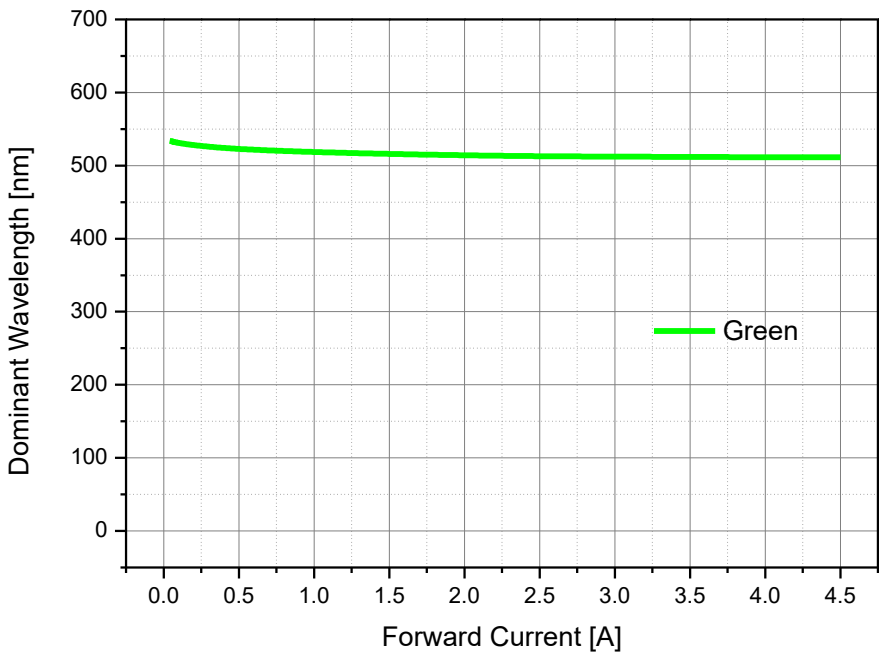
Forward Current vs Dominant Wavelength, Tj=25°C
