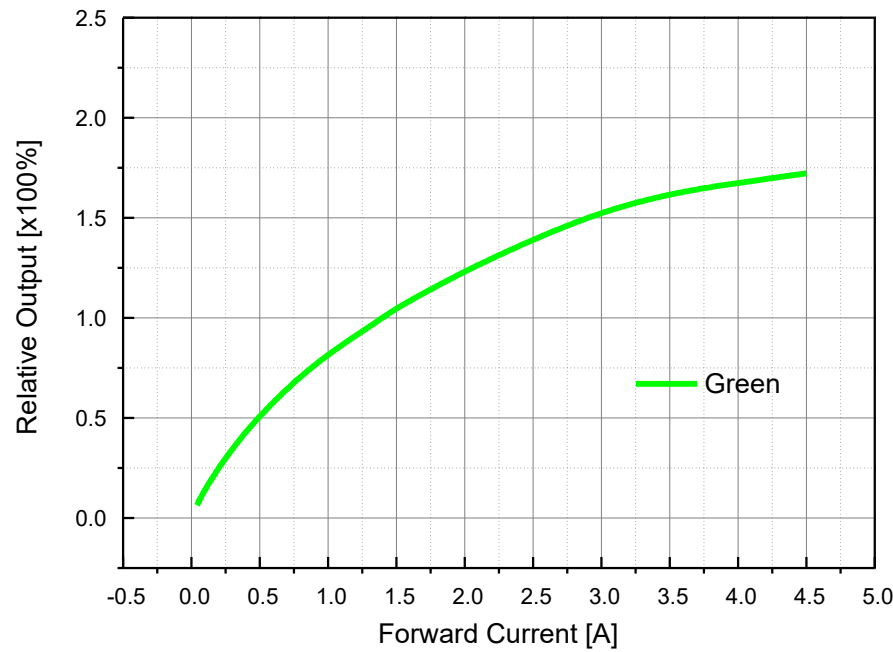
Forward Current vs. Normalized Relative Luminous Flux, Tj=25°C
