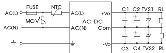
Fig. 2: LH20-10A series (Dual Output) typical application circuit
