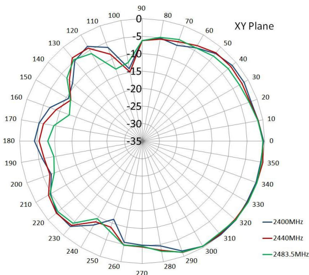
WIFI Antenna
