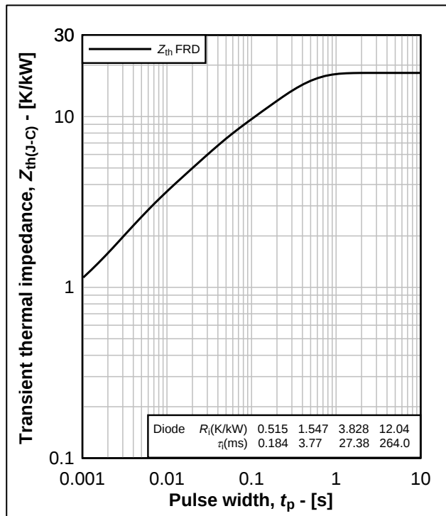
图 9. 瞬态热阻抗曲线, Z_{th(J-C)} = f(t_p)
