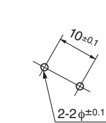
(PC board hole dimensions)
