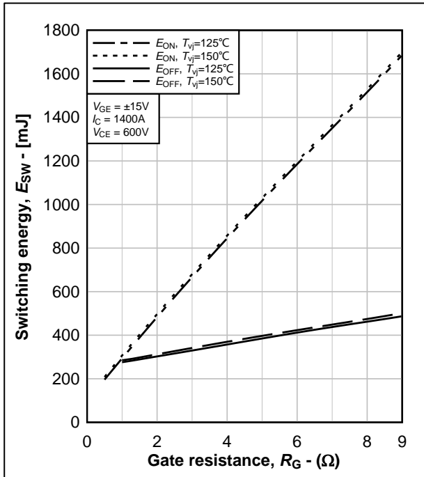
图 11. IGBT 开关能耗典型曲线, E_{on} = f(R_G) , E_{off} = f(R_G) Fig.11 Typical IGBT switching energy, E_{on} = f(R_G) , E_{off} = f(R_G)
