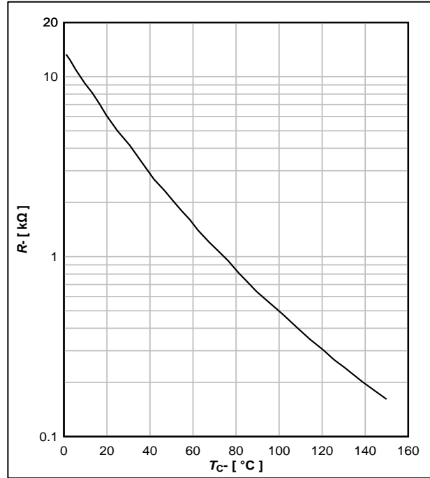
图 12. 热敏电阻典型特性曲线, R = f(T_C) Fig.12 Typical NTC thermistor characteristic, R = f(T_C)
