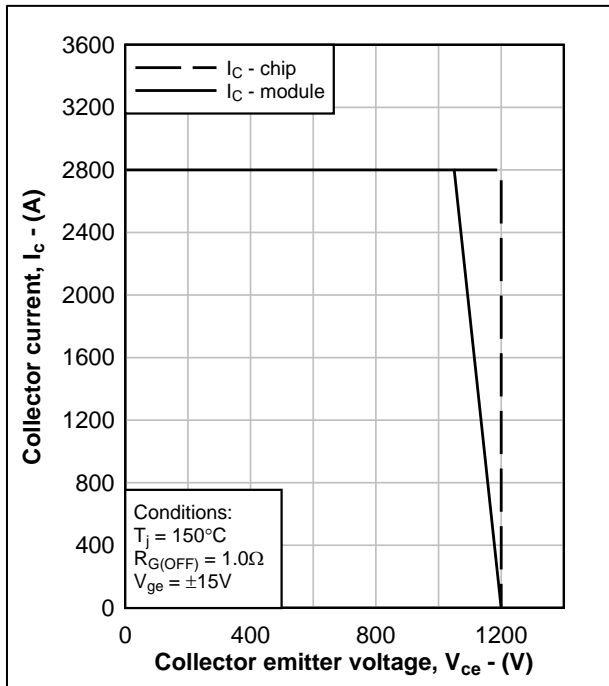
图 13. IGBT 反偏安全工作区, I_c = f(V_{CE}) Fig.13 Reverse bias safe operating area of IGBT, I_c = f(V_{CE})
