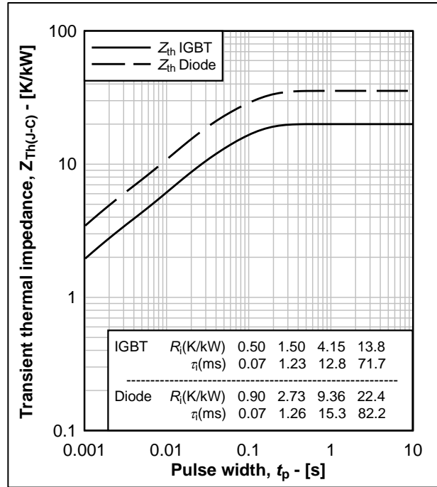
图 14. 瞬态热阻抗曲线, Z_{Th(J-C)} = f(t) Fig.14 Transient thermal impedance, Z_{Th(J-C)} = f(t)
