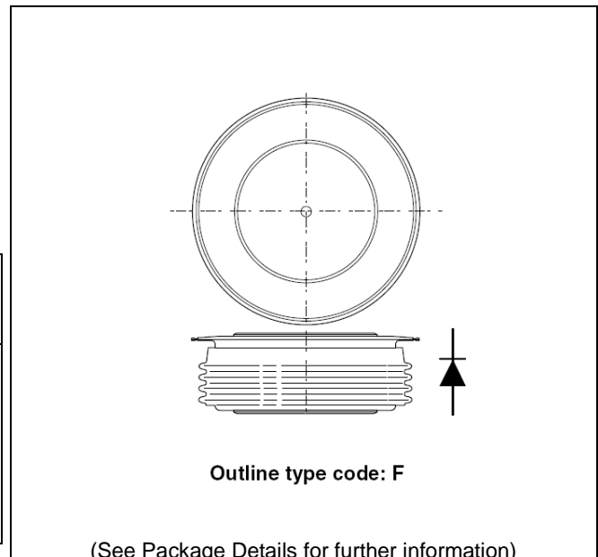
Fig. 1 Package outlines
